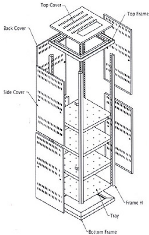
EXPLOSION VIEW
